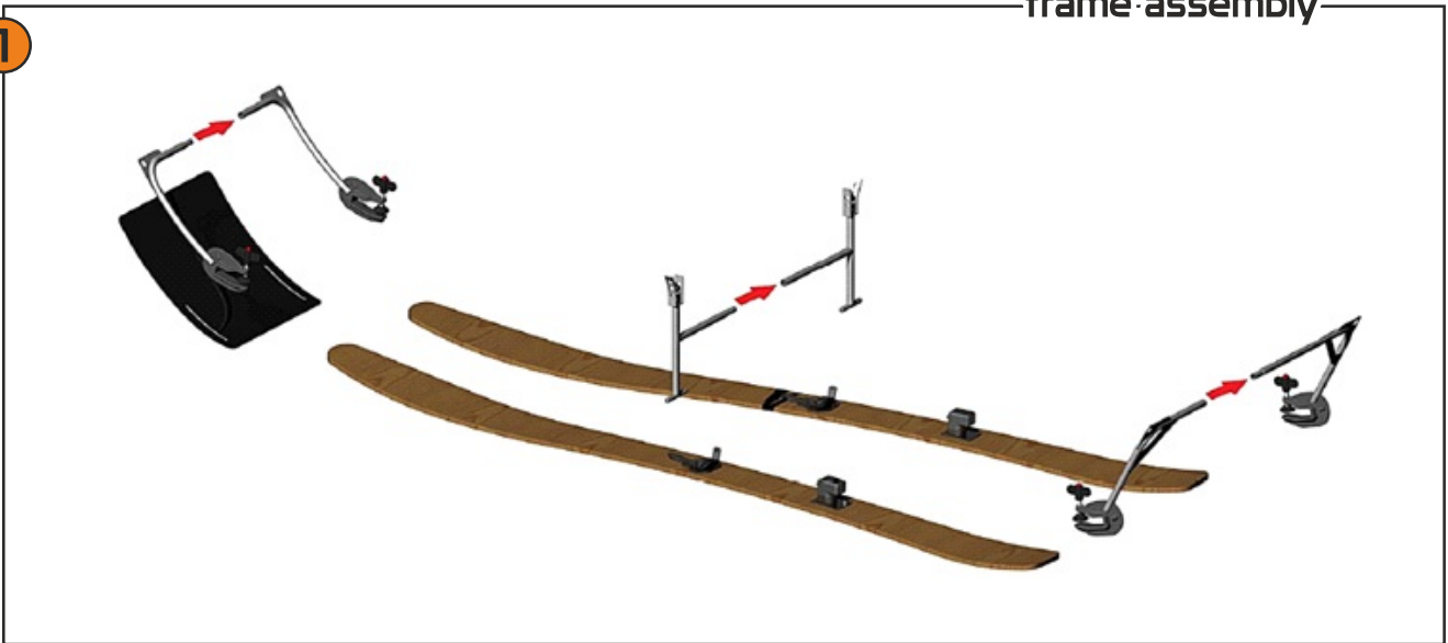
assembly-frame-on-sky
