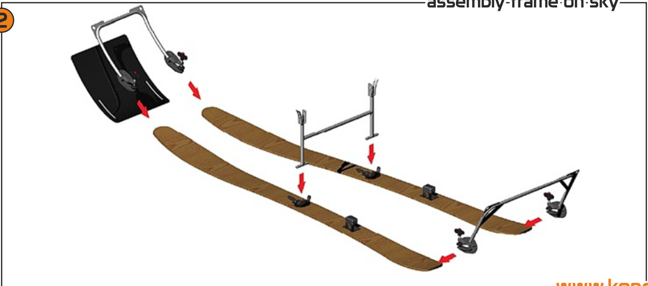
assembly-frame-on-sky
